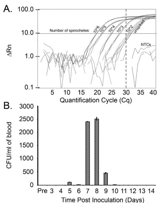
Figure 9. iPCR has the potential to directly detect B. burgdorferi in infected samples. (A) Live spirochetes were serially diluted in HN buffer (10 6 -10 2 spirochetes) and tested in triplicate using iPCR to detect organism capture using anti- B. burgdorferi antibody coated magnetic beads. A call threshold was assigned at greater than or equal to five times the standard deviation (Cq = 30, vertical broken line) above the mean background signal, as determined using HN buffer alone (unspiked). PCR non-template controls (NTCs) included water and TBST used during the iPCR protocol. (B) Six mice were prebled (pre) and inoculated intradermally with 1x10 5 B. burgdorferi strain B31 A3. Approximately 50 \mu l of blood/mouse was collected every day from groups of two mice every three days over a time period of 14 days. Blood collected from each mouse was plated in solid medium using 50 \mu l of blood and supplemented with a Borrelia antibiotic cocktail (see Materials and Methods for details) and the number of colony forming units (cfus) per ml of blood determined. Data shown are the average cfus/ml for the two mice sampled at each time point.
