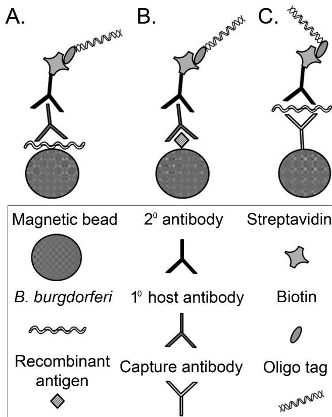
Figure 4. Schematic representation of iPCR assay for detection of Lyme disease biomarkers. (A) Intact spirochete or (B) recombinant protein antigen coupled to magnetic beads was used to capture B. burgdorferi -specific host generated antibodies. A biotinylated DNA oligonucleotide reporter molecule coupled to a streptavidin conjugated reporter antibody was amplified by qPCR for detection and quantification. (C) Anti- B. burgdorferi antibody coupled to magnetic beads was used for spirochete capture with detection accomplished by qPCR amplification of the DNA oligonucleotide coupled reporter antibody similar to detection of host antibody.
